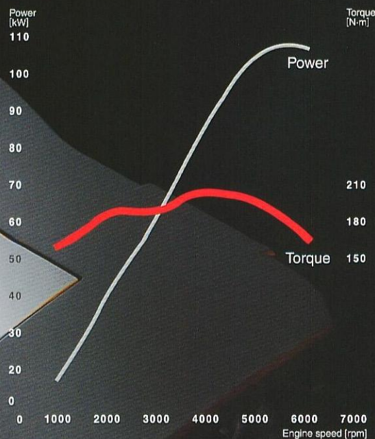
2.2 DOHC 16 VALVE[Z22] 108kW (147ps) / 5800rpm 203N·m (20.7kg·m) / 4000rpm
